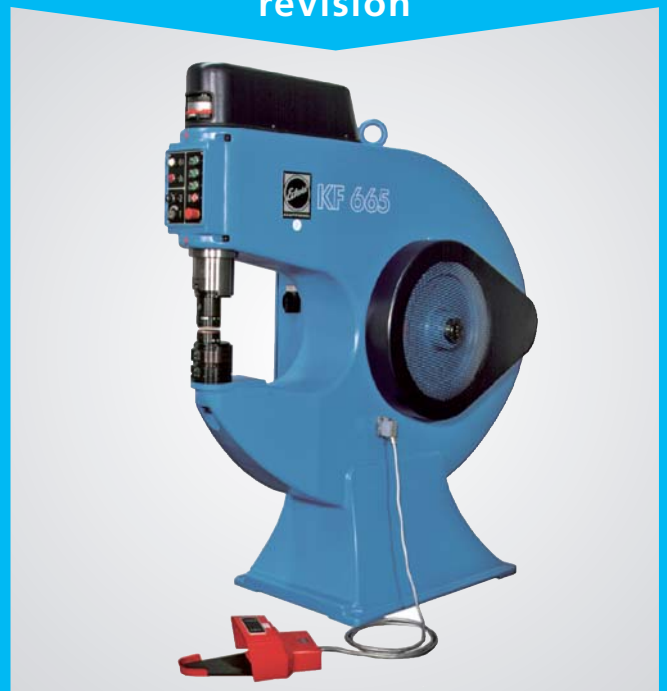
Kraftformer after the complete revision
